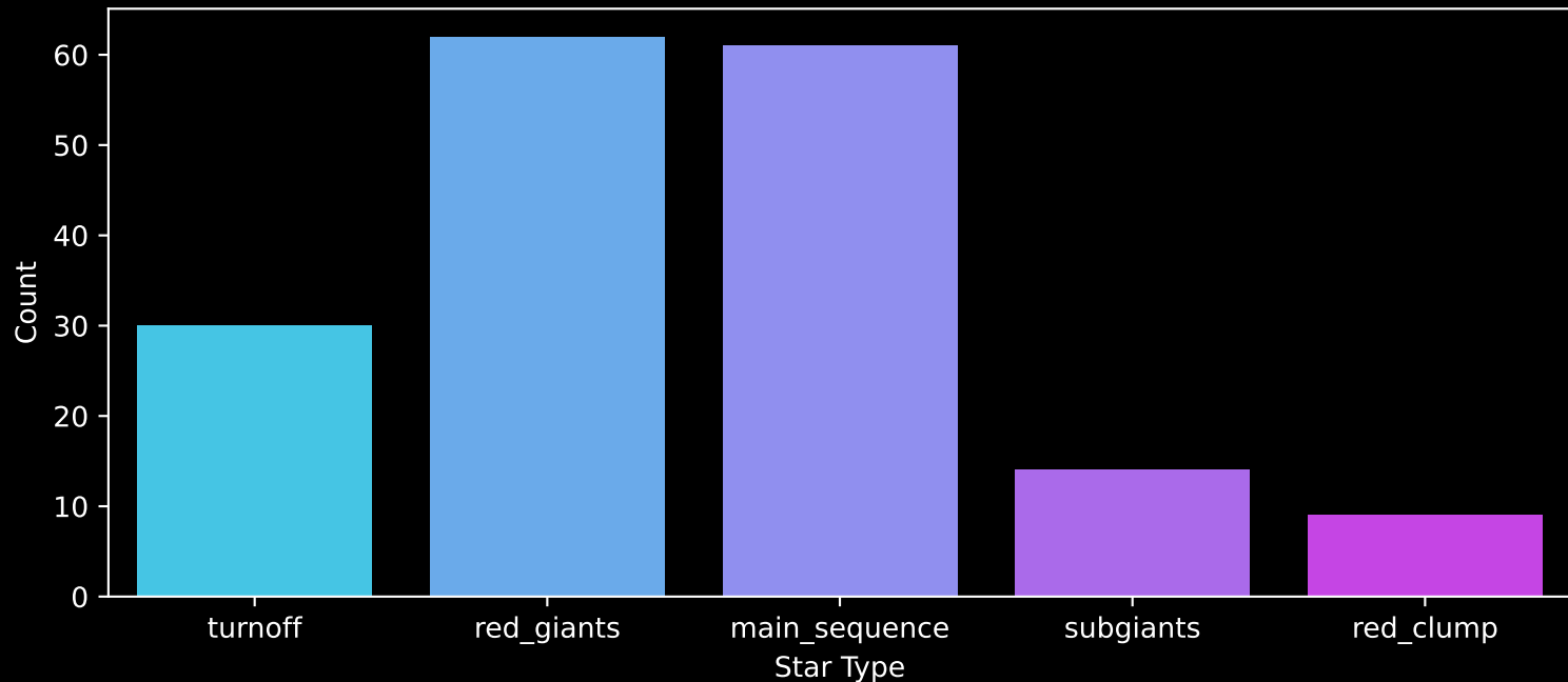
APOGEE DR17 Field: [CVZTILE_102+25_btx] Count plot of Star Type
