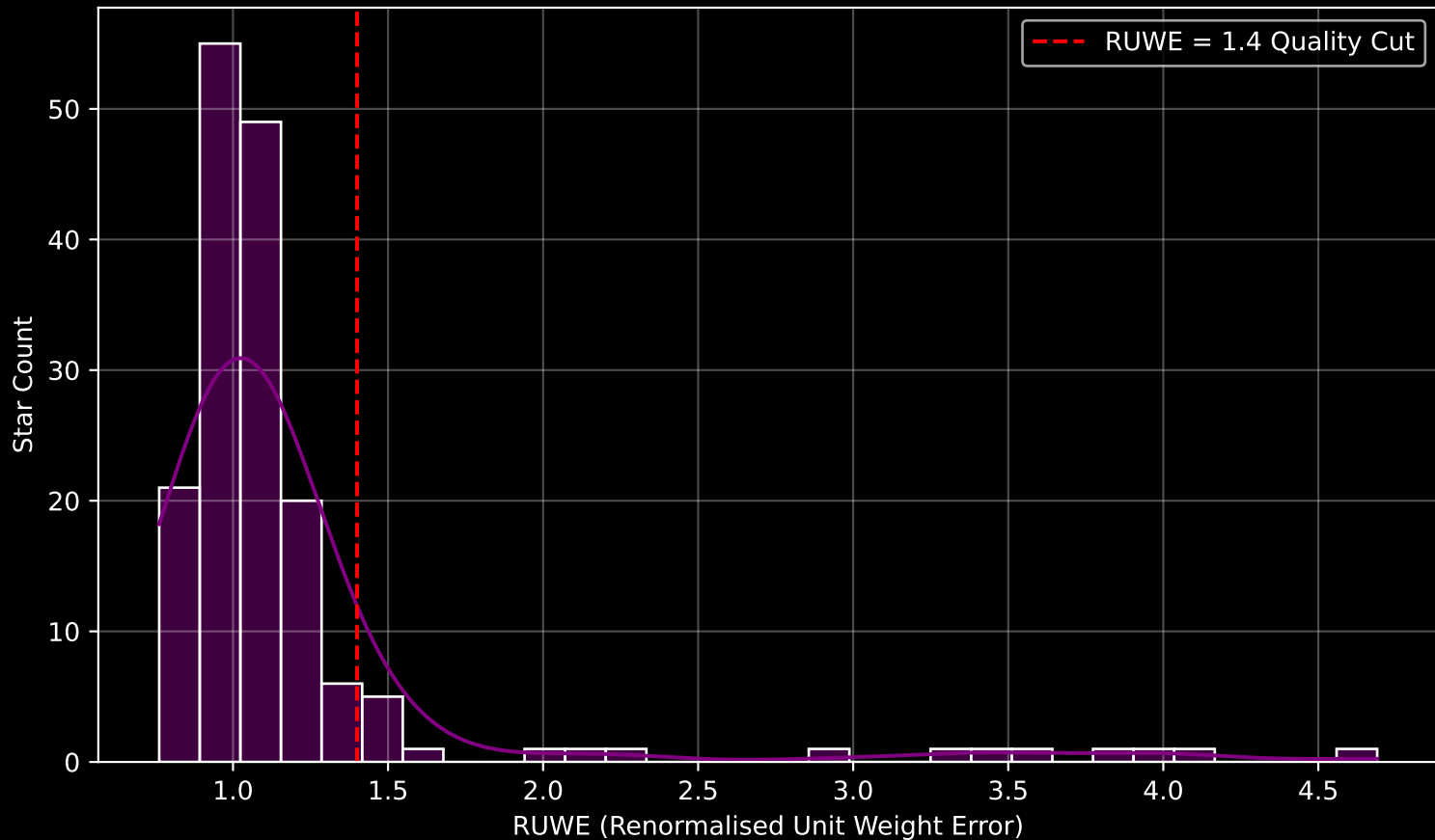
GAPOGEE DR17 Field [CVZTILE_102+25_btx] RUWE Distribution (n= 168)
