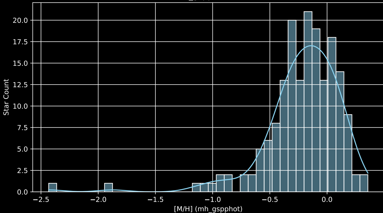
APOGEE DR17 Field: [CVZTILE_102+25_btx [M/H] (mh_gspphot) (n= 176)
