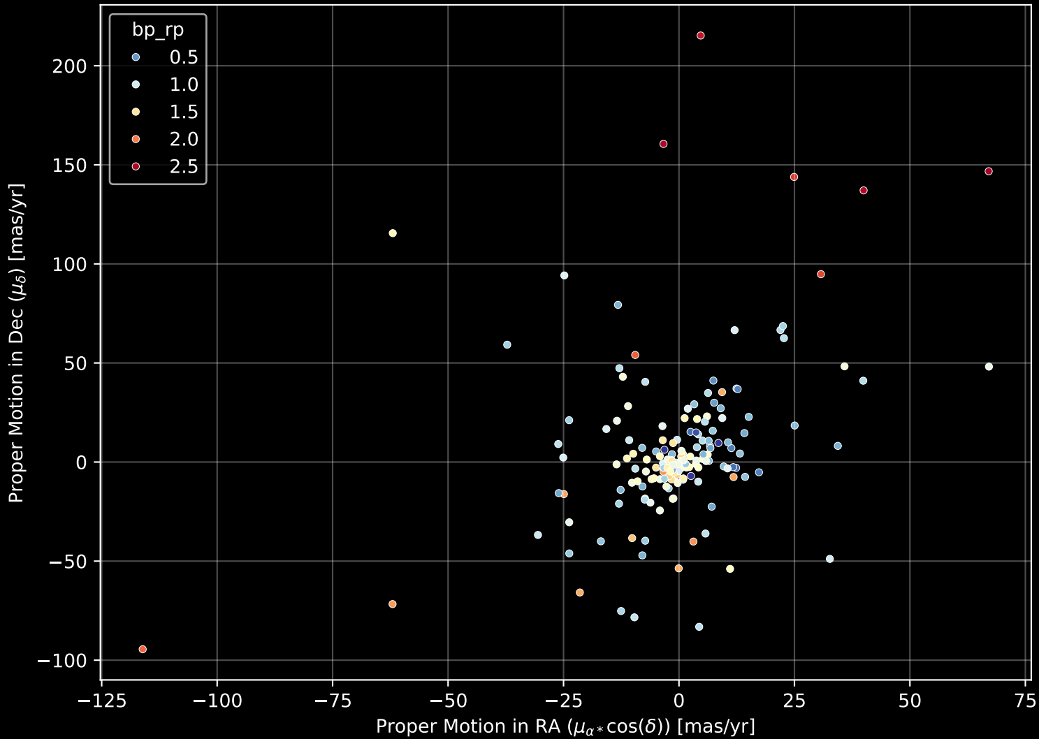
APOGEE DR17 Field: [CVZTILE_102+25_btx] Proper Motion Diagram (n= 176)
