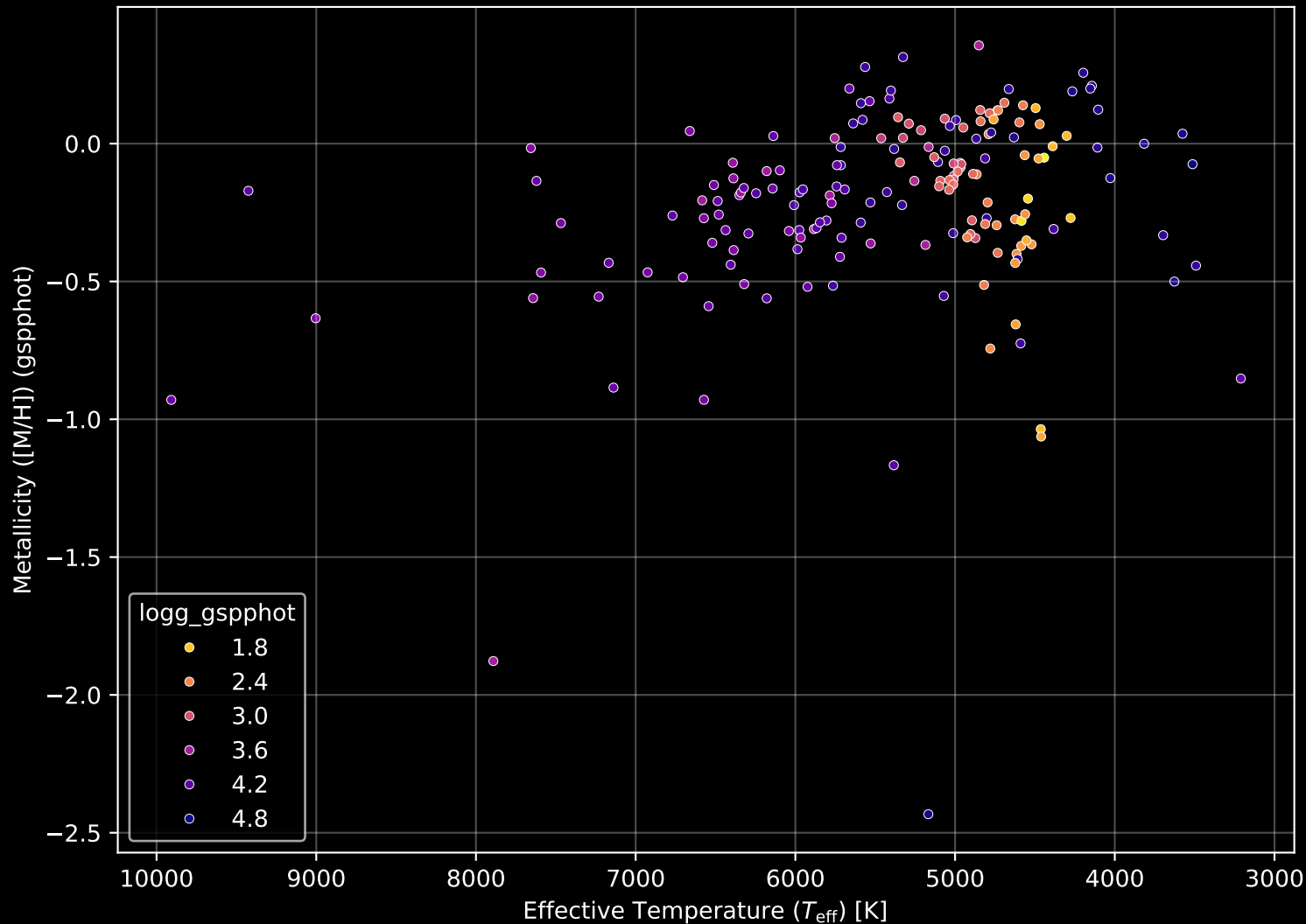
APOGEE DR17 Field: [CVZTILE_102+25_btx] Stellar Population Parameters (n= 176)
