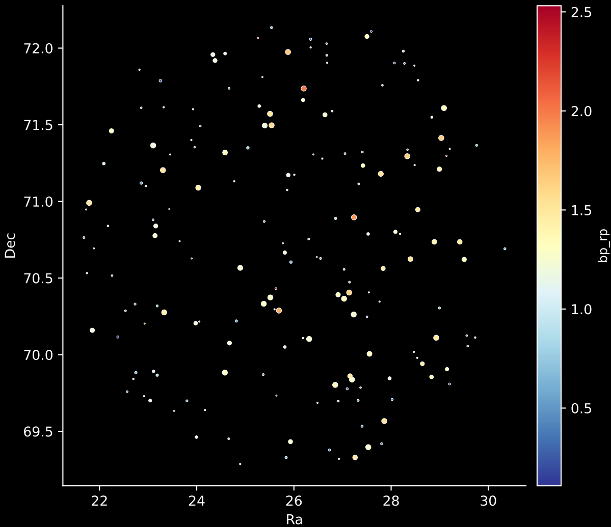
APOGEE DR17 Field: [CVZTILE_102+25_btx] Stars: 176
