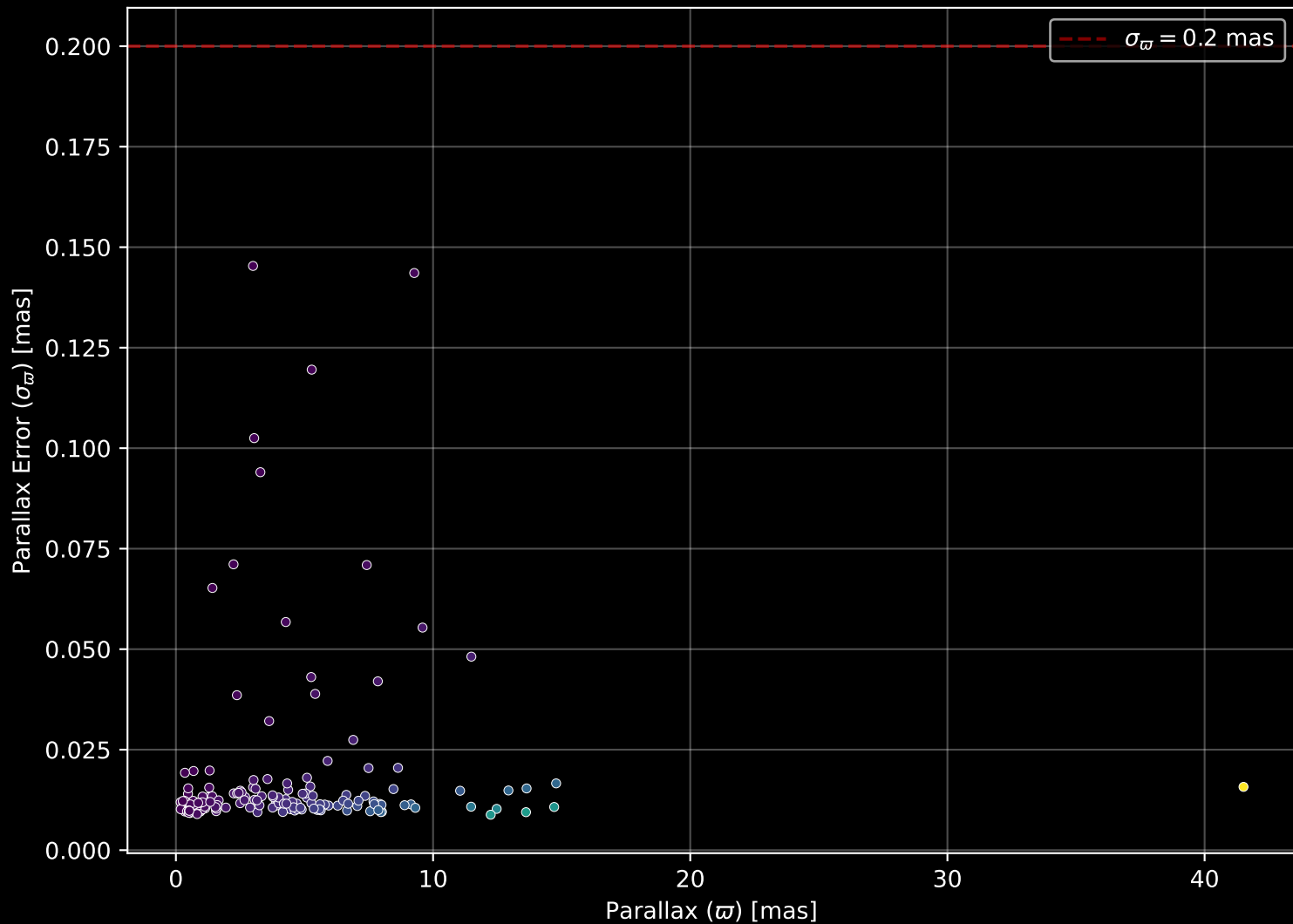
APOGEE DR17 Field: [CVZTILE_102+25_btx] Parallax Quality (n= 176)
